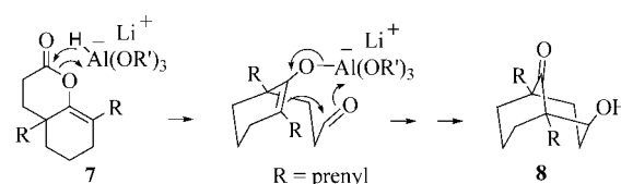
Scheme 3. Possible mechanism for the formation of the axial exo alcohol 8 .
