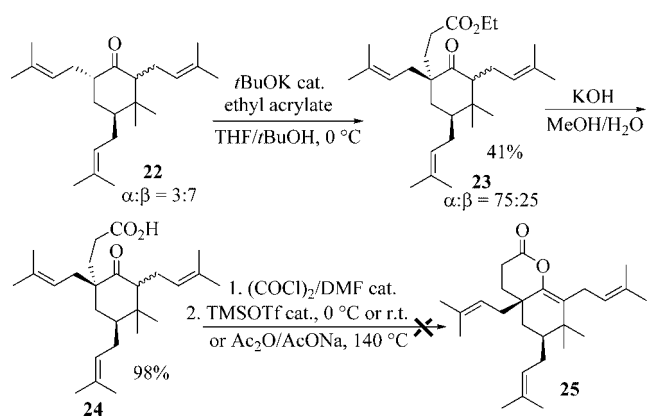
Scheme 6. Failure of enol lactone 25 formation.
