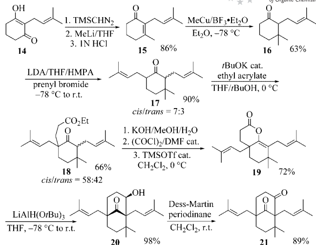
Scheme 5. Access to the 8,8-dimethyl-1,5-diprenyl bicyclic system.
