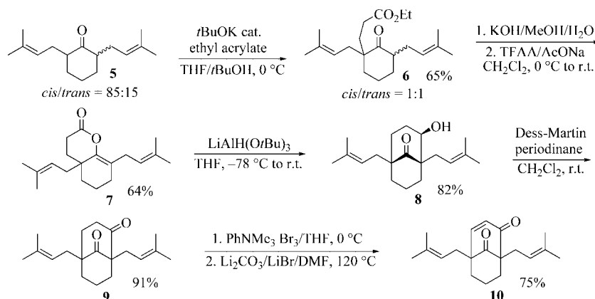
Scheme 2. Formation of bicyclic aldol compound 8 by reductive rearrangement of 7 .
