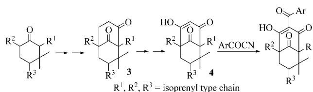
Scheme 1. Synthetic plan towards type B polyprenylated benzoylphloroglucinols.
