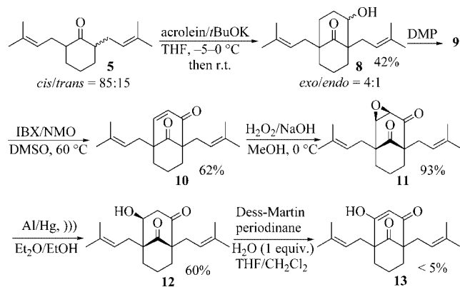
Scheme 4. \alpha,\alpha' -Annulation of 2,6-diprenylcyclohexanone with acrolein and further oxidation.
